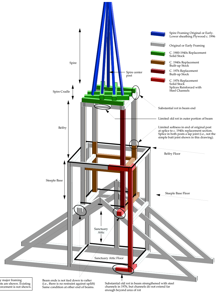
3.2: Three dimensional drawing of principal steeple framing as viewed from front with primary structural issues noted. Age of various past replacement timbers is indicated by colors.
